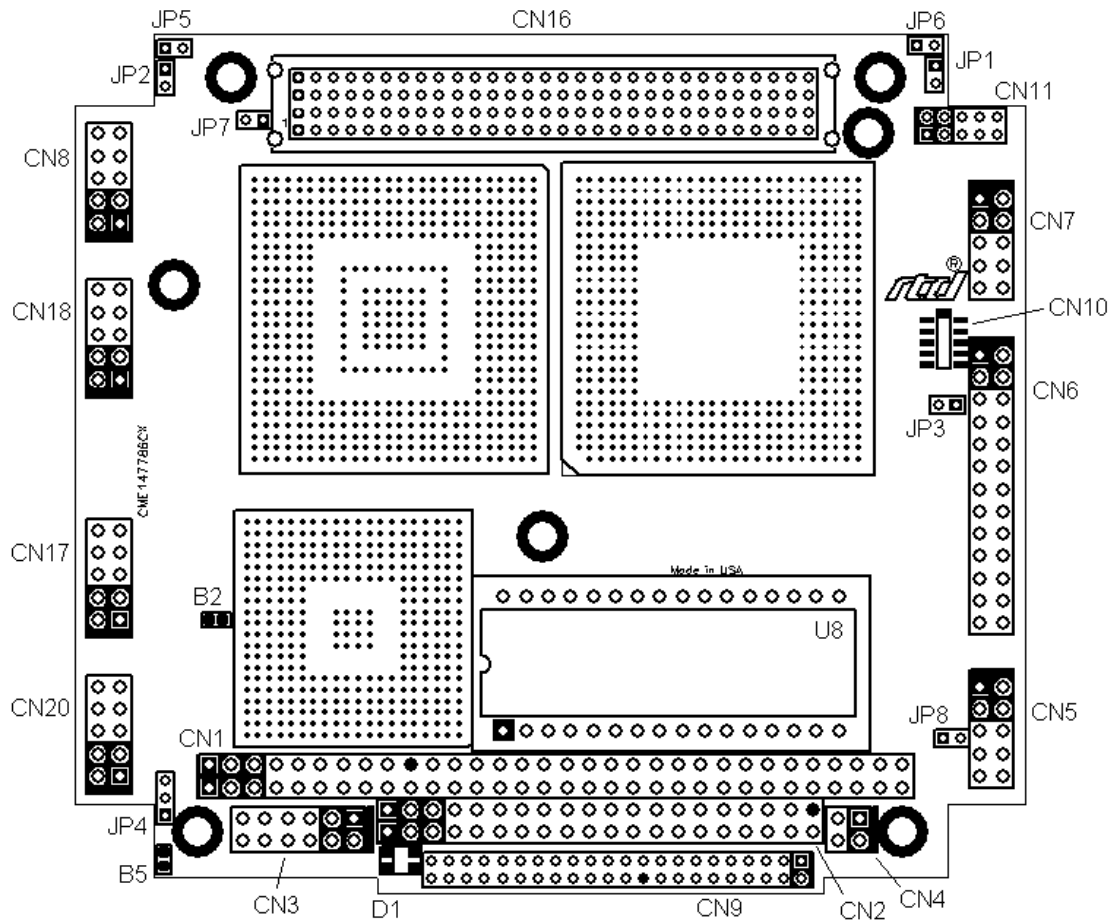
Figure 3: CME147786CX Connector Locations
