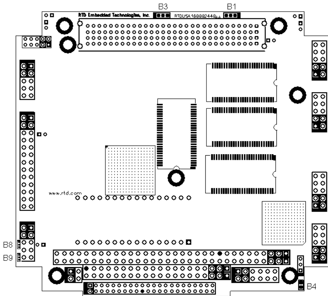
Figure 5: CME147786CX Jumper Locations - Bottom
