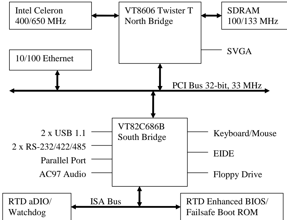
Figure 1: CME147786CX Block Diagram
