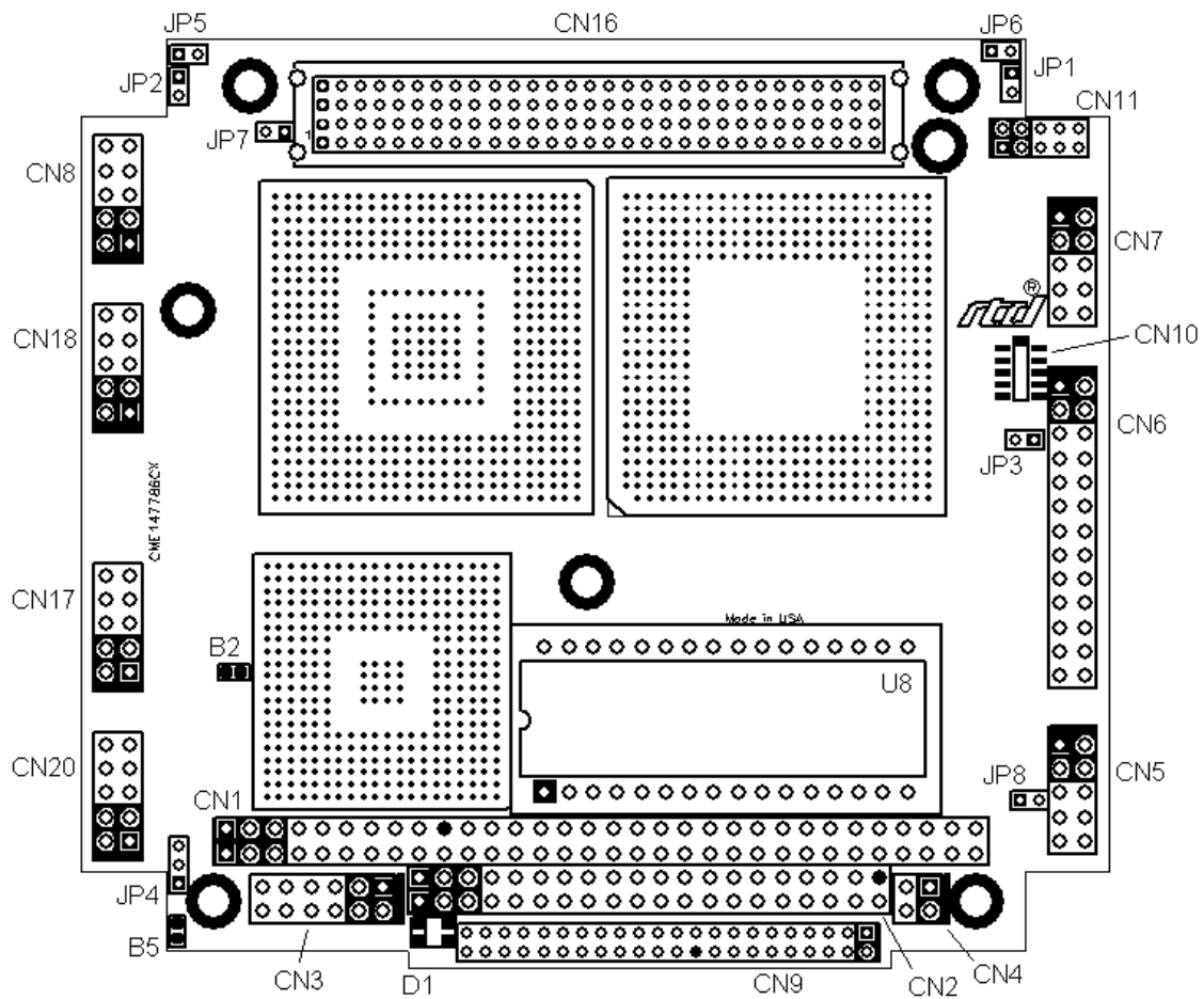
Figure 4: CME147786CX Jumper Locations - Top
