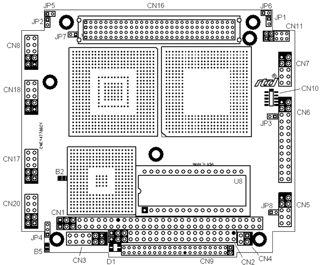
Figure 2: CME147786CX Basic Connector Locations
