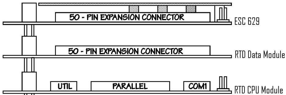
Fig. 3-1: ESC629 integrated into a PC/104 RTD cpuModule stack
