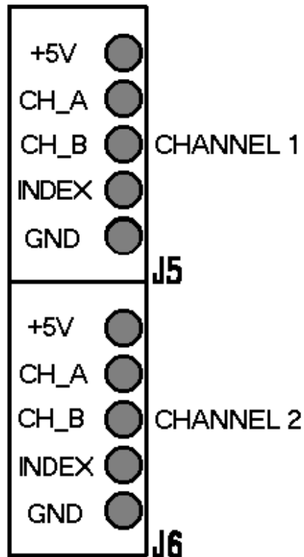
Fig. 3-3 Incremental encoder terminal-blocks
