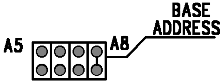
Fig. 2-2: Base address jumpers illustrating address 300H
