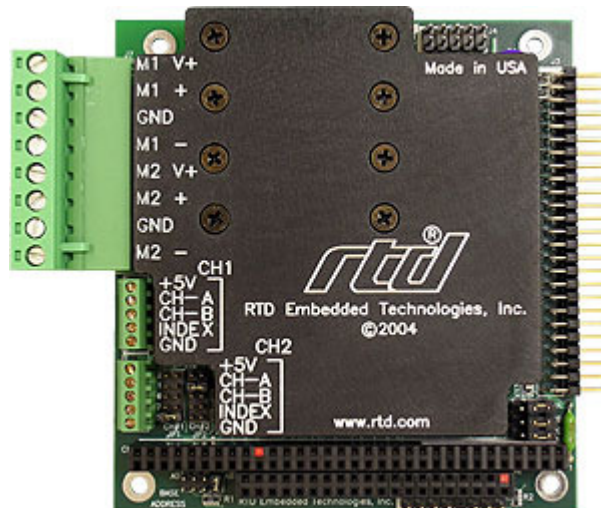
Figure 2-1: ESC629 Board layout showing jumper locations
