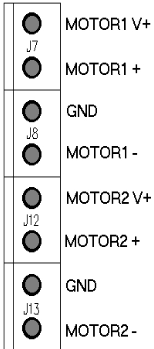
Fig. 3-2 Motor interface terminal block
