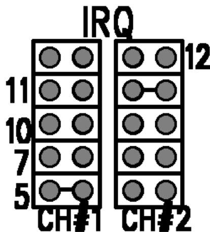
Fig. 2-3: Interrupt jumpers
