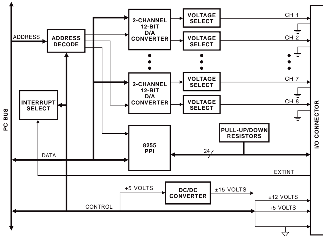
Fig. 3-1 — DM5604 Block Diagram
