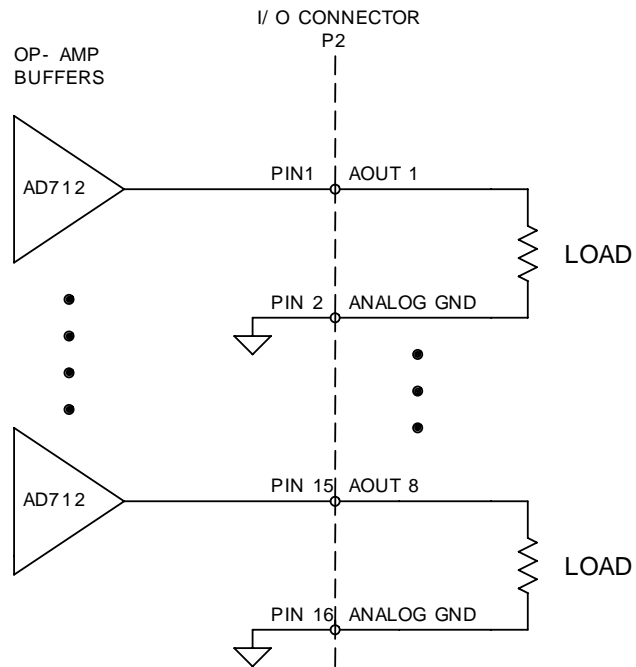
Fig. 2-2 — Voltage Output Connections
