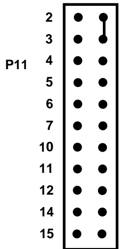
Fig. 1-3 — Interrupt Channel Select Jumper, P11
