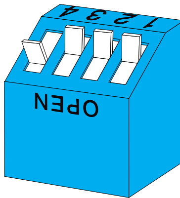
Fig. 1-6 — Base Address Switch, S1
