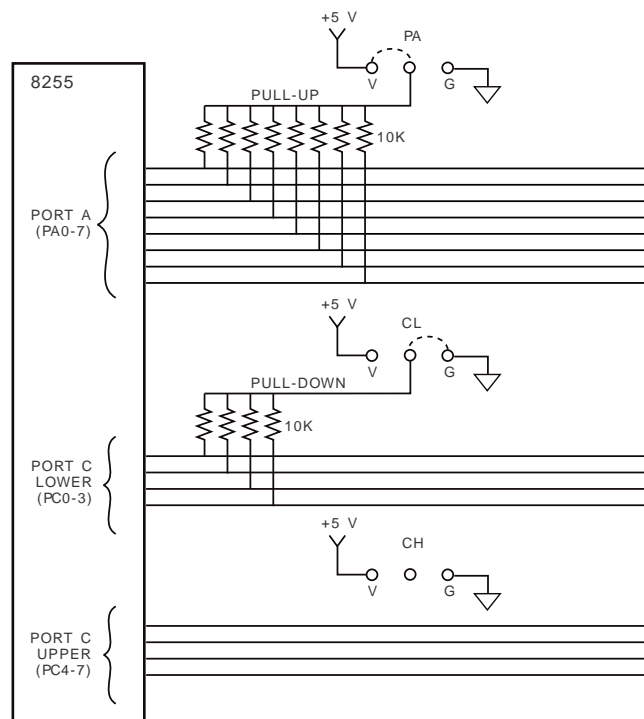
Fig. 1-8 — Adding Pull-ups and Pull-downs to Some Digital I/O Lines
