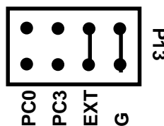
Fig. 1-4 — Interrupt Source Select Jumpers, P13
