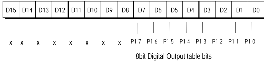
Figure 4.2.2. Digital Output Table bits
