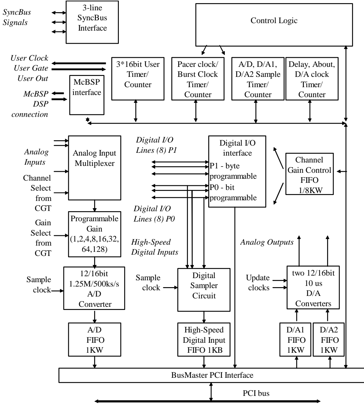
Figure 1.1. PCI4520/DM7520/DM7530 Block Diagram
