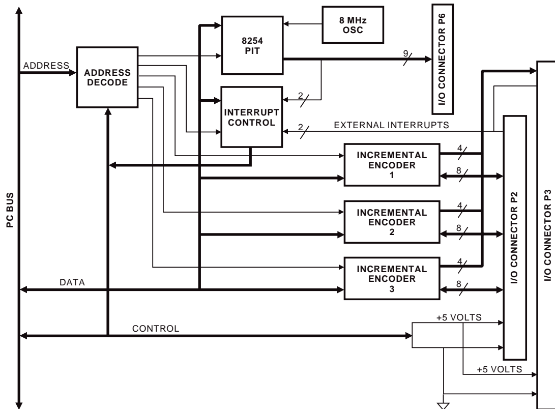
Fig. 3-1 — DM5814 Block Diagram
