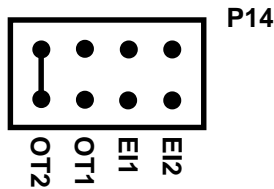
Fig. 1-6 — Interrupt Source Select Jumper, P14
