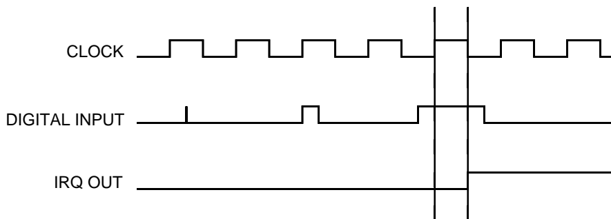
Fig. D-1 — Digital Interrupt Timing Diagram
