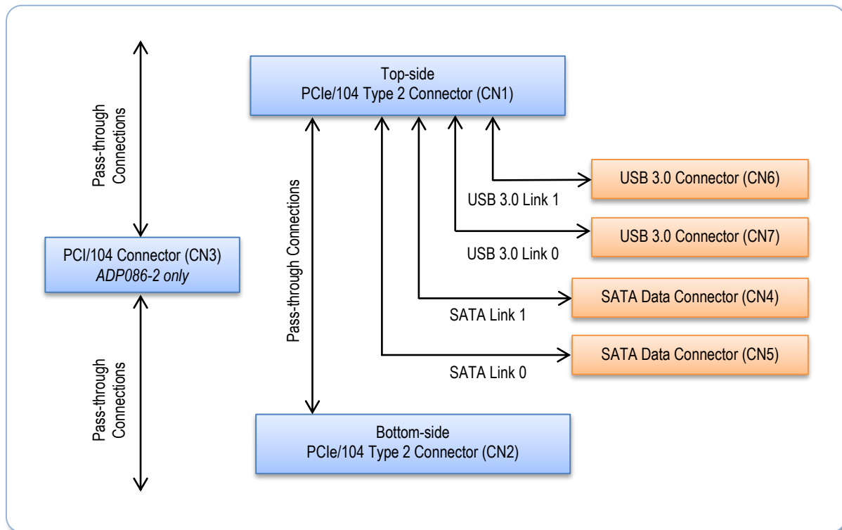
Figure 6: ADP086 Functional Diagram
