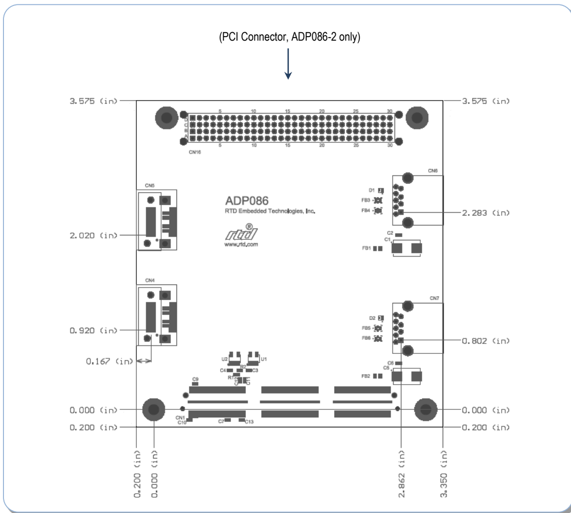
Figure 3: Board Dimensions (inches)
