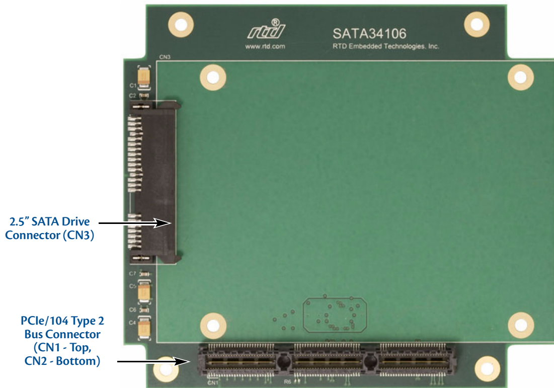
Figure 1 SATA34106 SATA Drive Carrier (top view)
