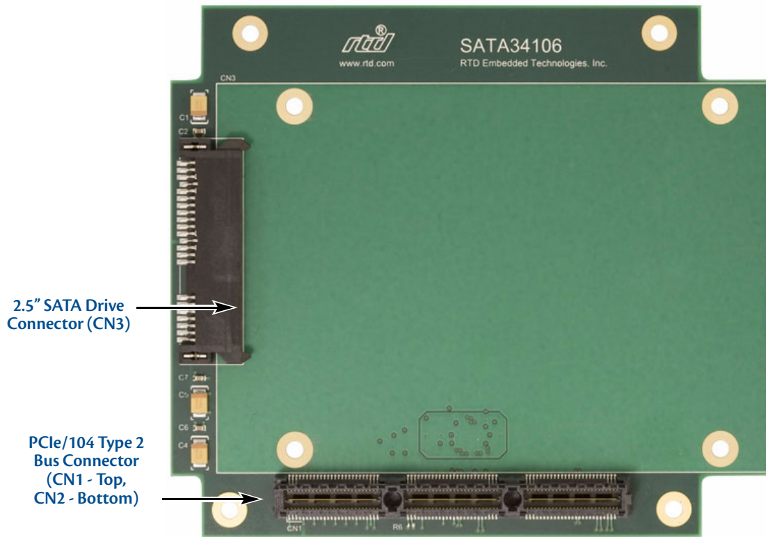
Figure 2 SATA34106 Connector Locations
