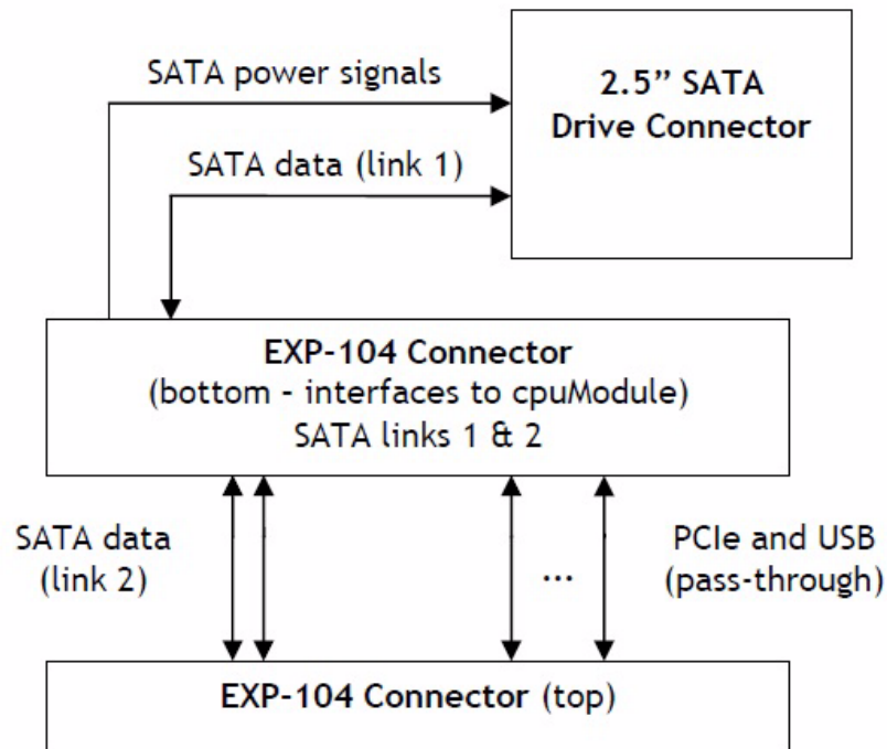
Figure 3 SATA34106 - Block Diagram
