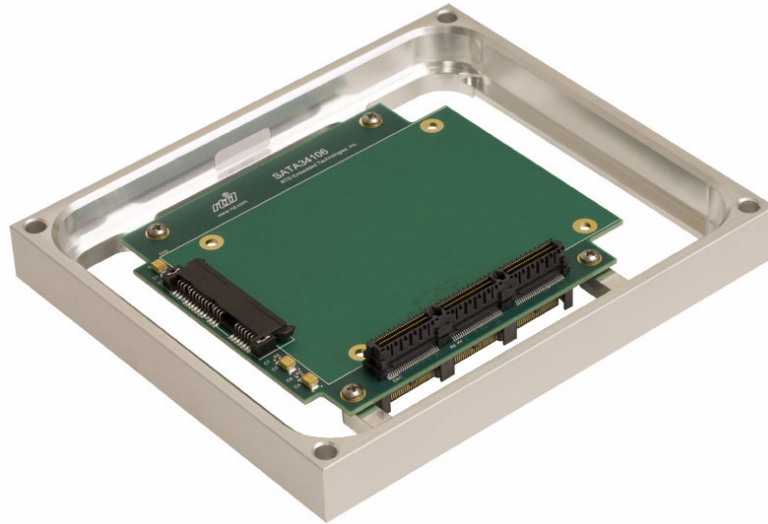
Figure 4 IDAN-SATA34106
